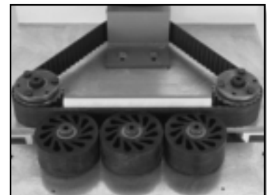
PE11 Conveyor Assembly
